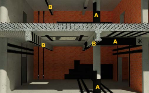
A Carbon Fiber Sheet for Shear Strengthening B Carbon Fiber Plate for Flexural Strengthening
